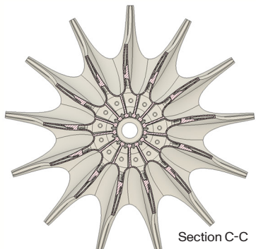
Figure 2. Internal structure within blades at various build heights
